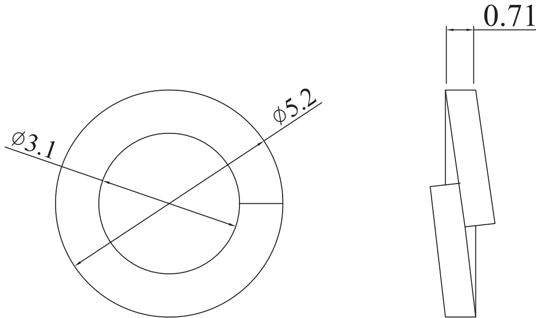
Split Washer
