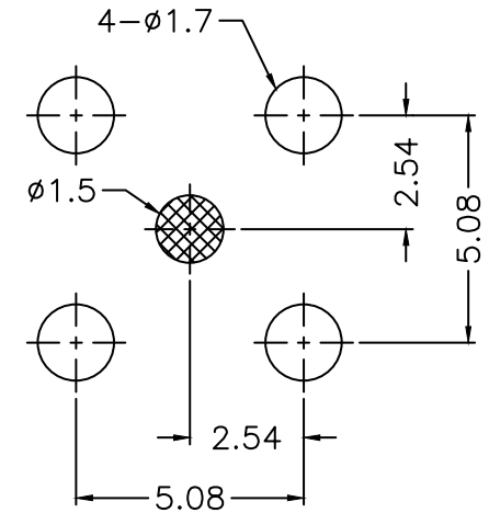
PCB MOUNTING HOLE (印刷电路板架設孔)
