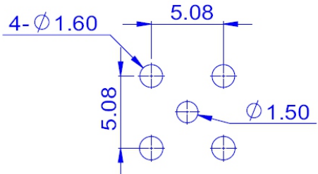
RECOMMENDED PC BOARD LAYOUT WITHOUT MOUNTING POSTS
