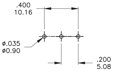
P.C. MOUNTING
