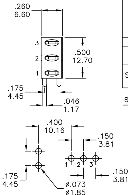
P.C. MOUNTING
