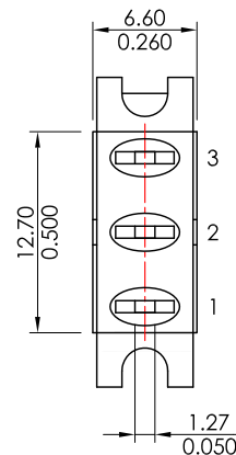
PANEL MOUNTING
