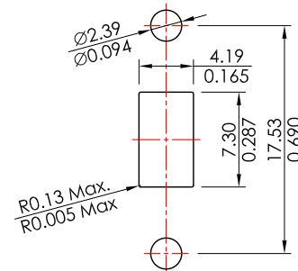
PANEL MOUNTING
