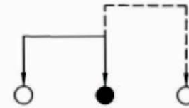
SCHEMATIC (NON-SHORTING)
