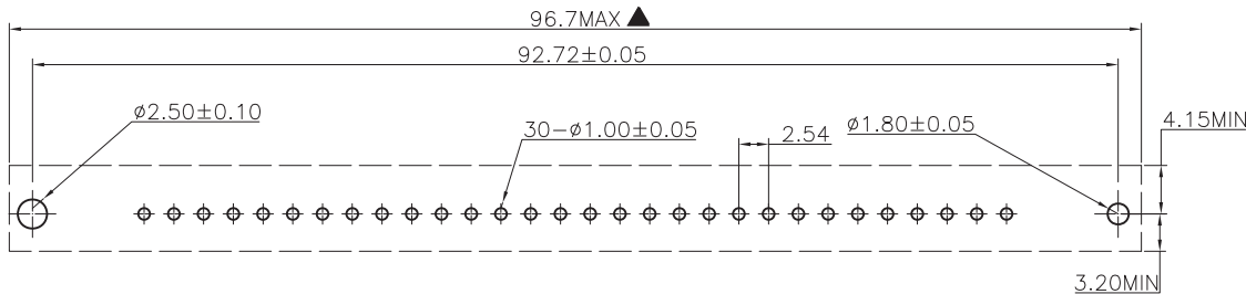
TOP VIEW PCB LAYOUT RECOMMENDED
