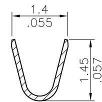
SEC. B-B SCALE 10/1
