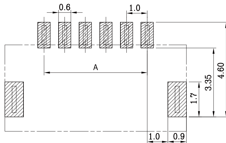
SHL-W-xx P.C. BOARD LAYOUT
