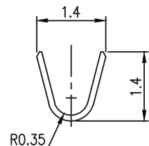
INSULATION BARREL
