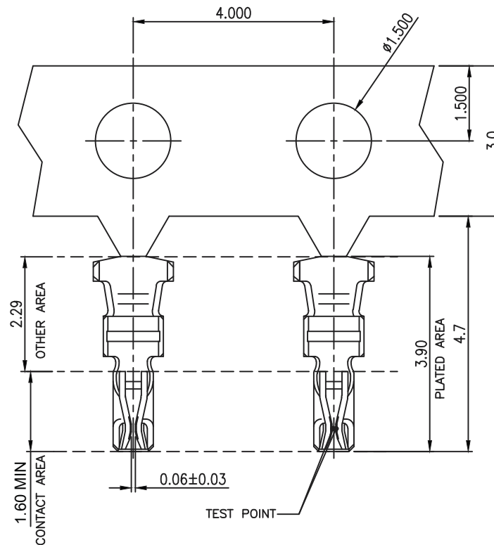
INSULATION BARREL
