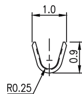
WIRE BARREL
