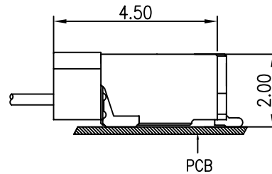
MATED CONDITION
