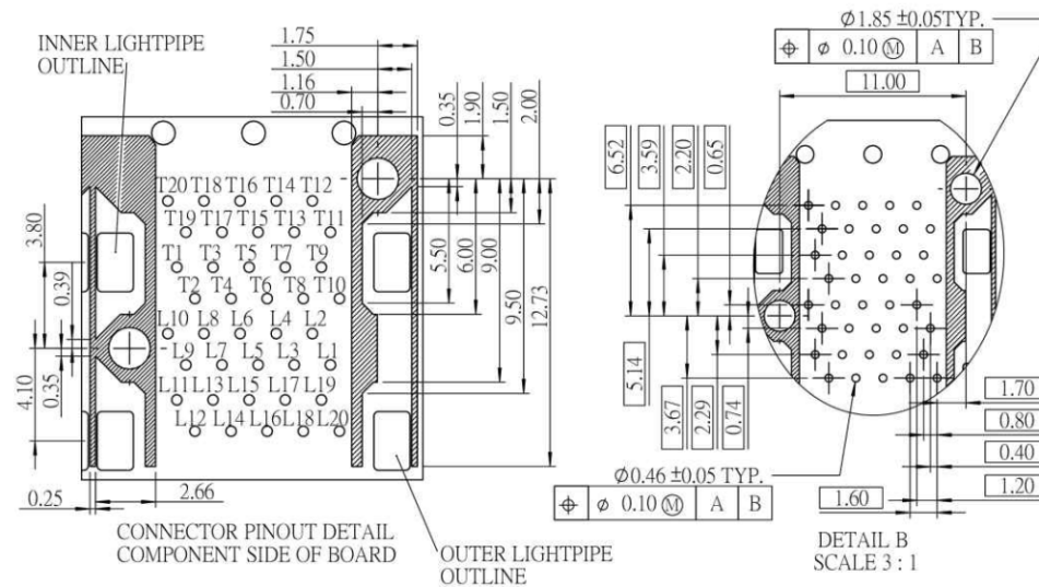
RECOMMENDED PCB CONFIGURATION
