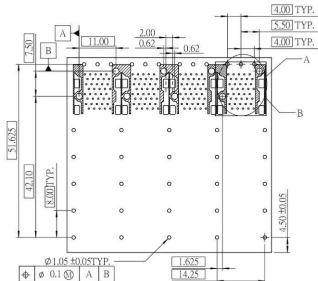
RECOMMENDED PCB CONFIGURATION
