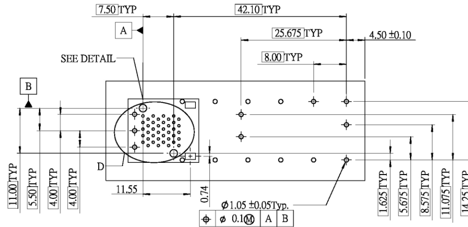
RECOMMENDED PCB CONFIGURATION
