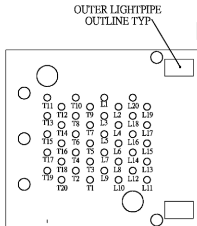
CONNECTOR PINOUT DETAIL COMPONENT SIDE OF BOARD
