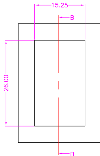
BEZEL CUT-OUT OPENING DETAIL
