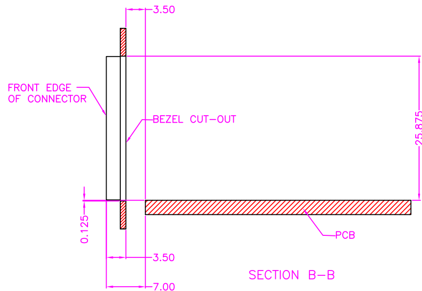
SECTION B-B BEZEL OPENING BELOW TIP OF PCB
