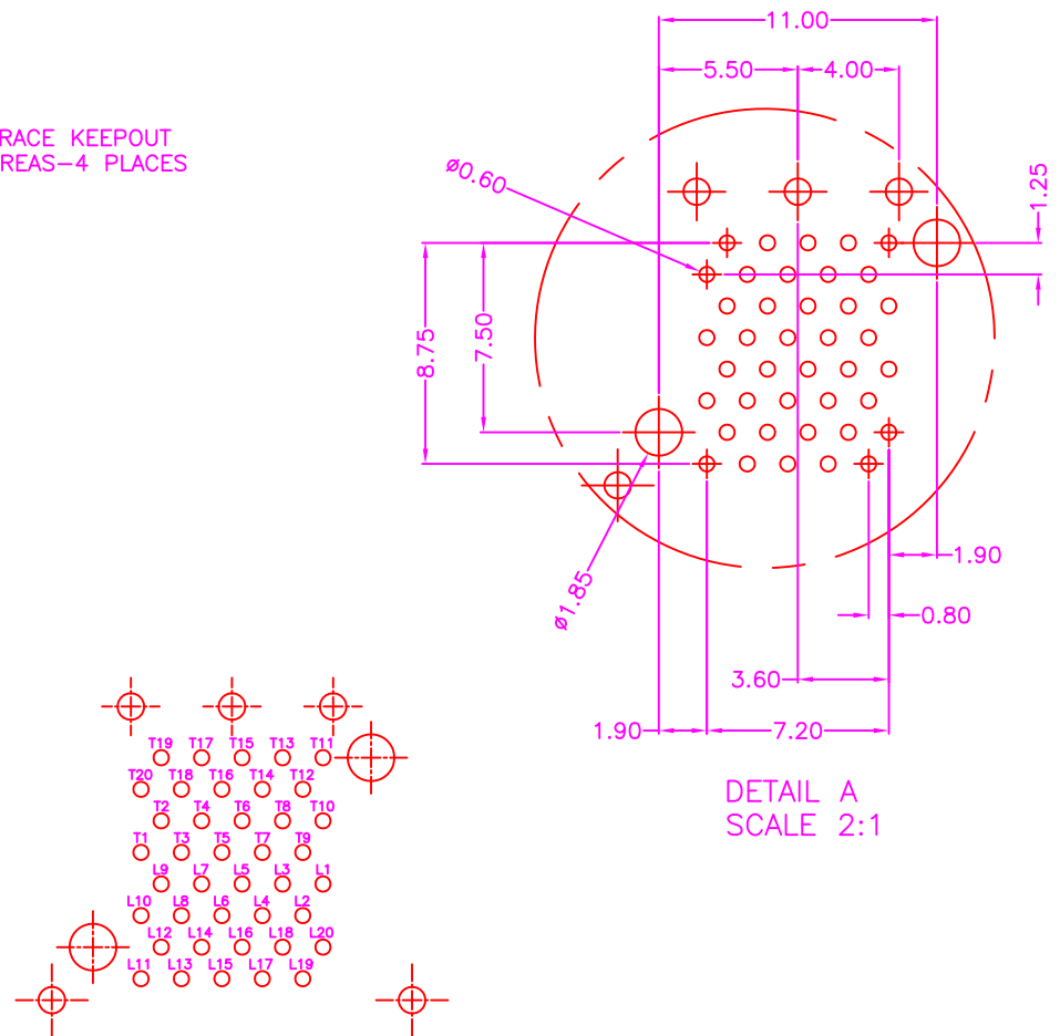
CONNETTON PINOUT DETAIL COMPONENT SIDE OF BOARD
