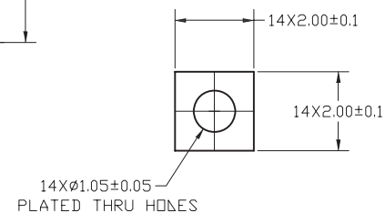
DETAIL B SCALE 4:1
