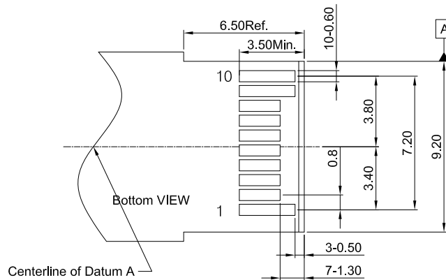
RECOMMENDED LAYOUT MATING PCB SIDE
