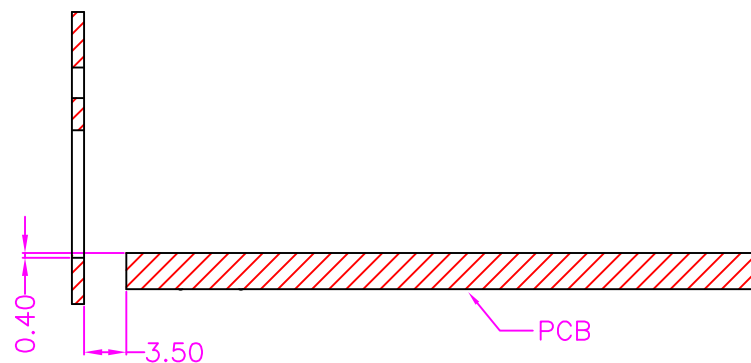
BEZEL OPENING BELOW TOP OF PCB
