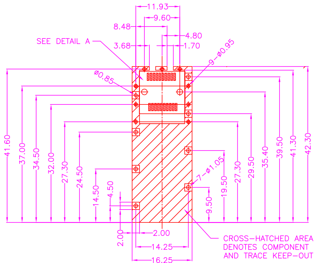
P.C.B LAYOUT TOP VIEW ±0.05
