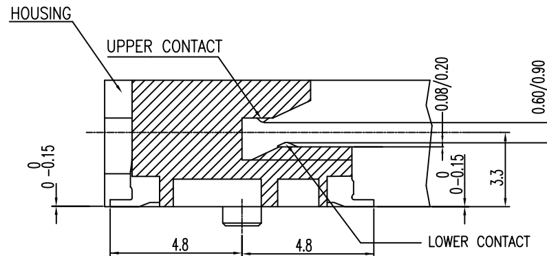
SECT "A"-"A" (S=4/1)
