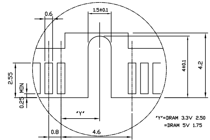
DETAIL X
