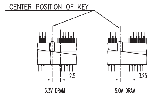
DETAIL FOR KEY POSITIONS
