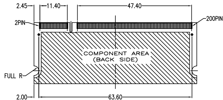
DDR SO-DIMM MODULE BOARD LAYOUT
