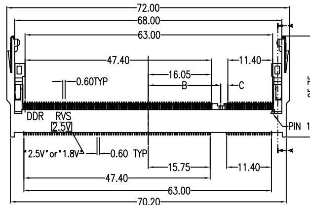
SECT:F-F
