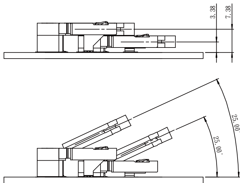
DDR S.O. DIMM 200P 5.2&9.2 OVERLAY FIGURE
