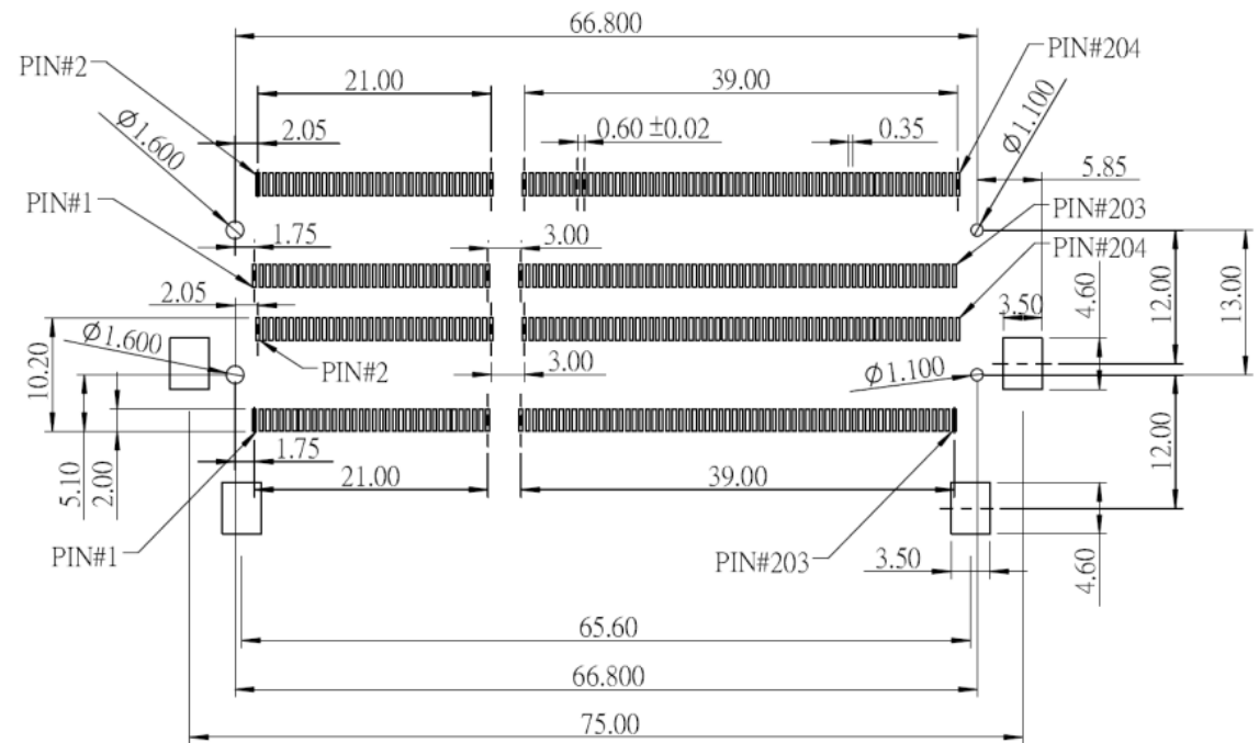
PCB LAYOUT
