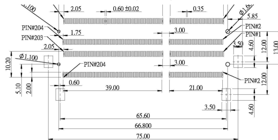
PCB LAYOUT : COMPONENT SIDE(5.2&9.2TYPE)
