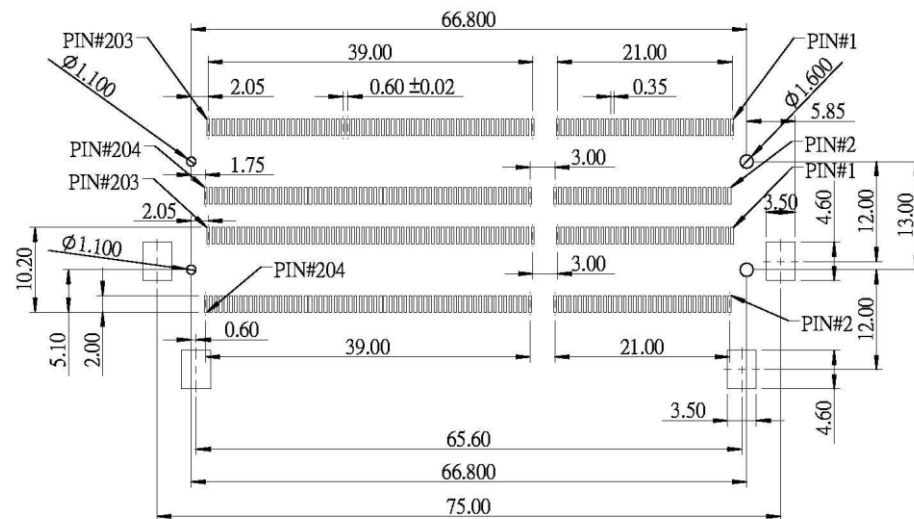
PCB LAYOUT : COMPONENT SIDE(5.2&9.2TYPE)
