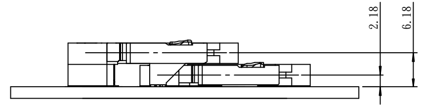
DDR S.O. DIMM 200P 4.0&8.0 OVERLAY FIGURE
