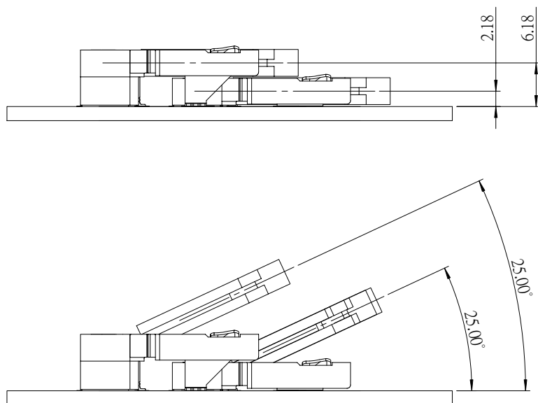
DDR S.O. DIMM 200P 4.0&8.0 OVERLAY FIGURE
