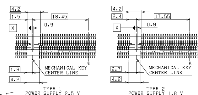
DETAIL C MECHANICAL KEY TYPE
