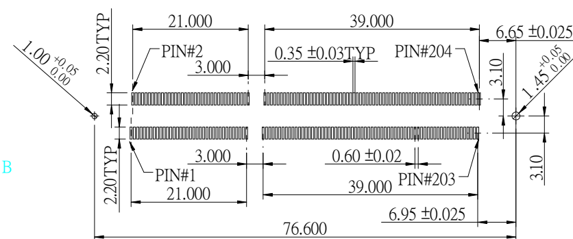
PCB LAYOUT
