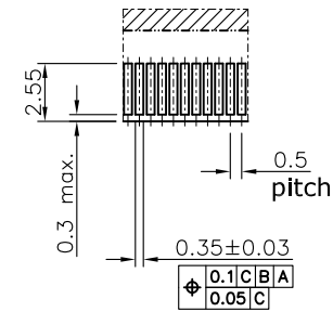
Detail D SCALE 3.125
