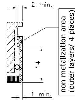
Detail F
