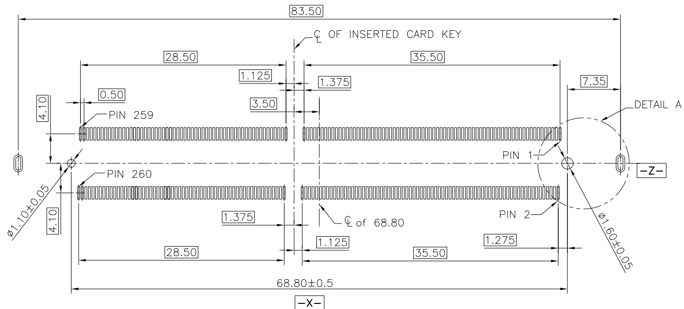
RECOMMENDED PCB LAYOUT (TOP VIEW) DEFAULT TOLERANCES:±0.05MM
