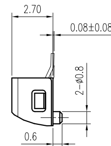
Detail 1 Scale 3.2:1
