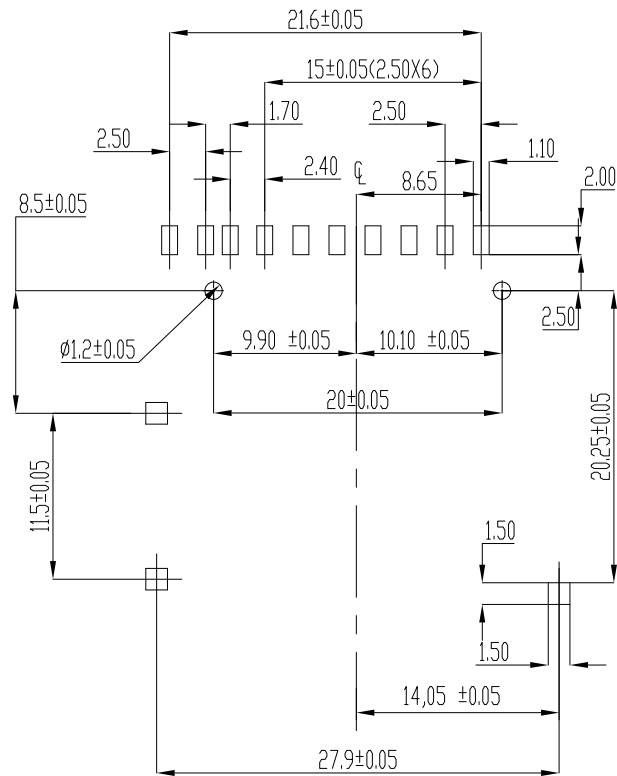
PCB LAYOUT (ALL TOLERANCE ARE ±0.05)
