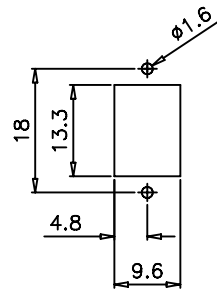
SUGGESTED PANEL CUTOUT
