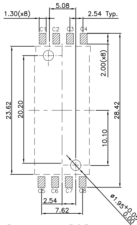
Recommended P.C.B Layout Component Side (Tolerance: \pm 0.05 )
