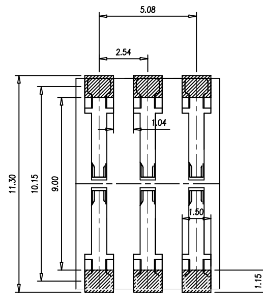
PCB PAD LAYOUT
