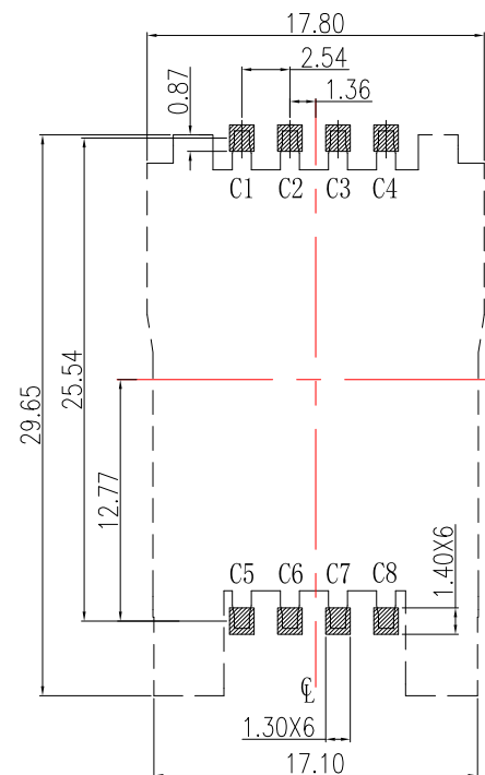
RECOMMENDED PCB LAYOUT TOLERANCE: \pm 0.05
