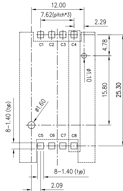
PCB LAYOUT TOLERANCE: 0.05mm
