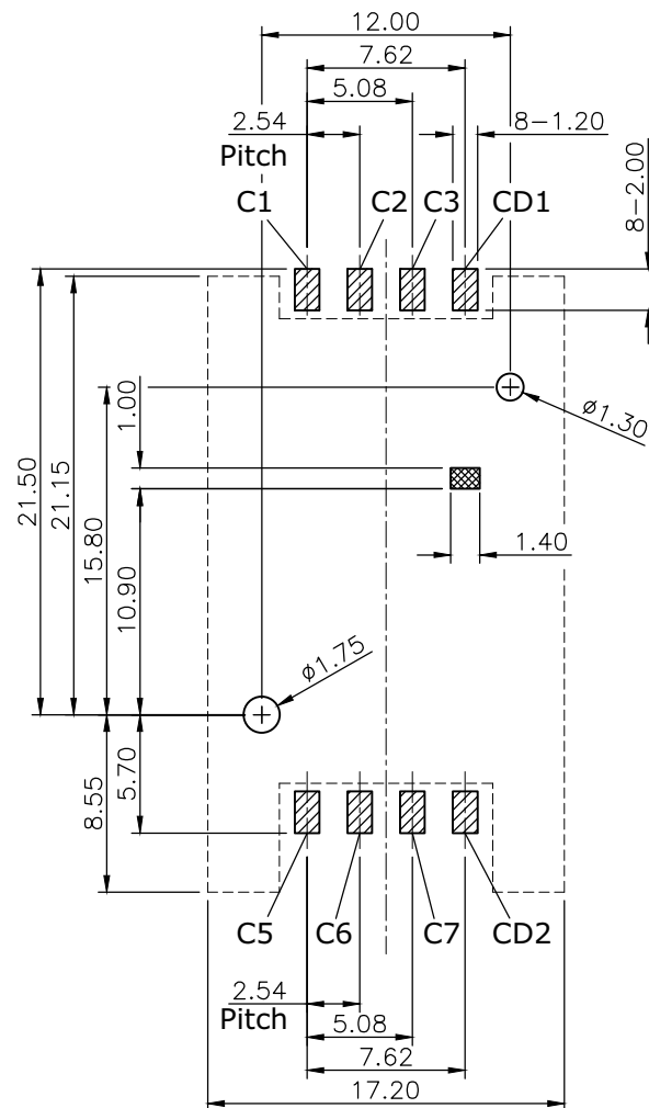
RECOMMENDED LAYOUT (TOP VIEW) GENERAL TOLERANCE: \pm 0.05
