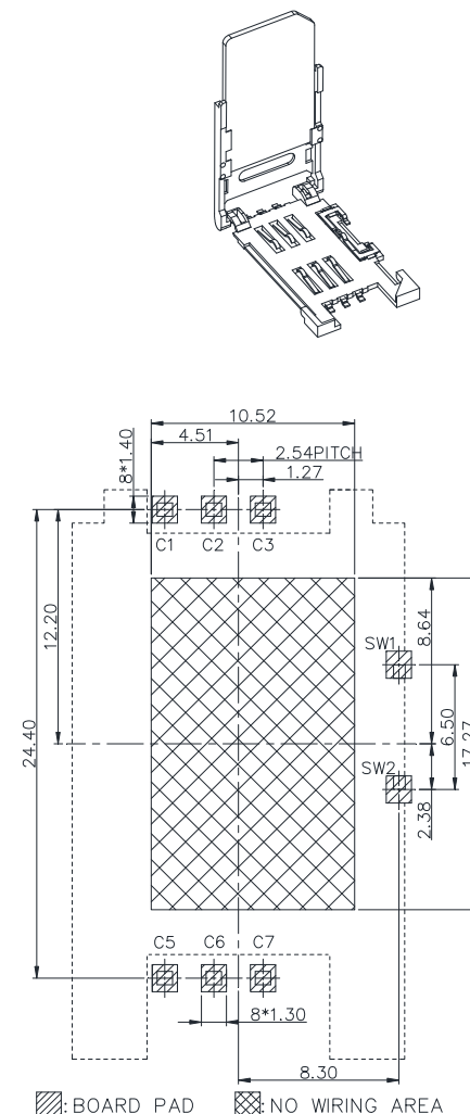
Unit: mm; Tolerances: \pm 0.05 mm Reference dimension for PCB layout
