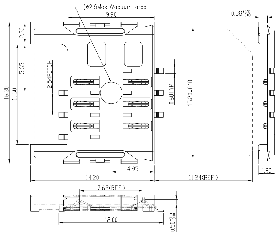
Figure 5.1 Mechanical outline dimension (6 pins)
