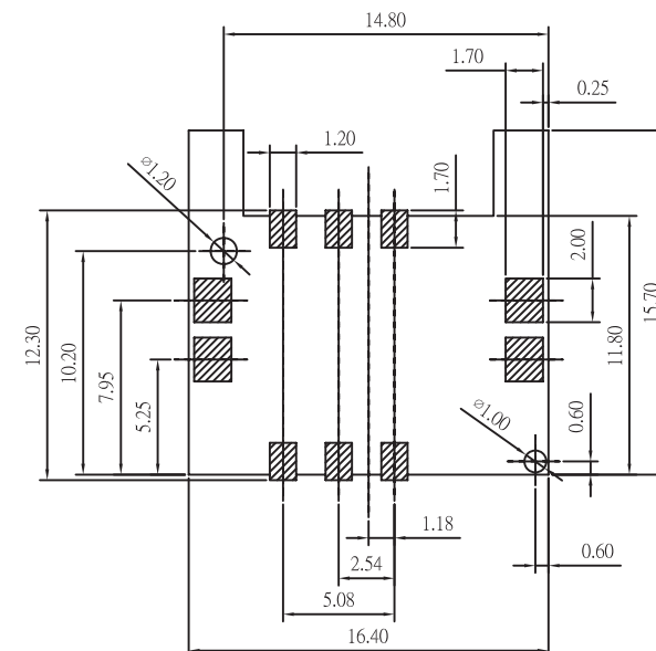
RECOMMENDED PC BOARD LAYOUT TOLERANCE: \pm 0.05\text{mm} [TOP VIEW]
