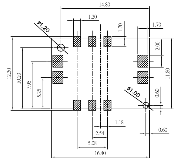
RECOMMENDED PC BOARD LAYOUT TOLERANCE: \pm 0.05\text{mm} [TOP VIEW]
