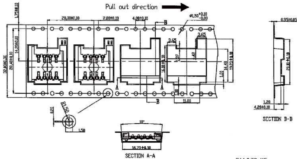
5.1.2 Reel Form Diagram
