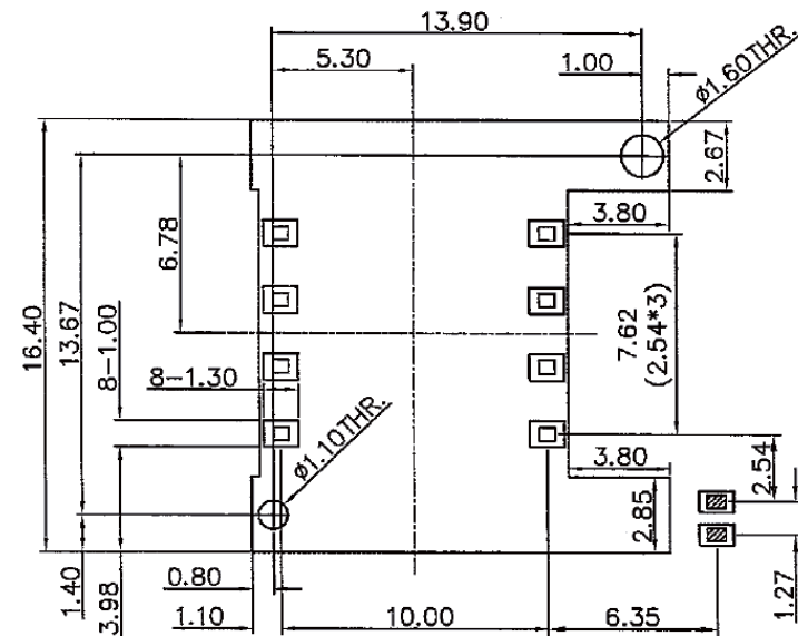
P.C.B. LAYOUT (TOLERANCES:±0.10mm)
