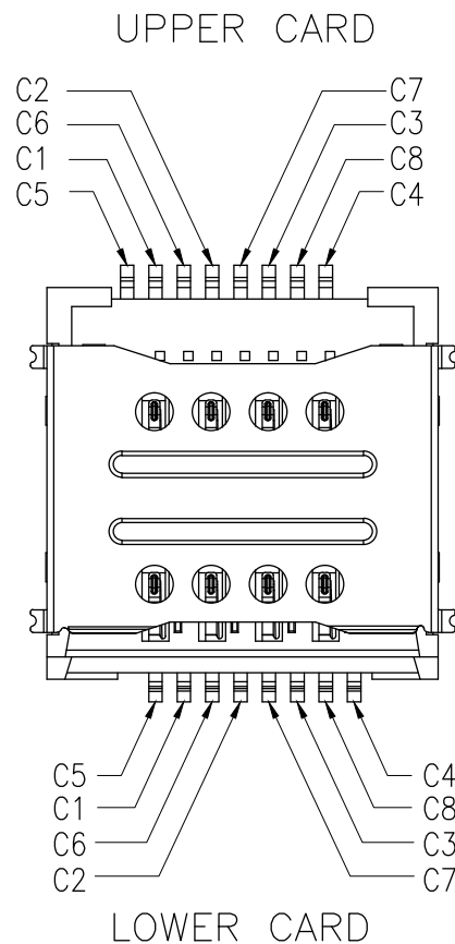
SIM CARD CIRCUIT
