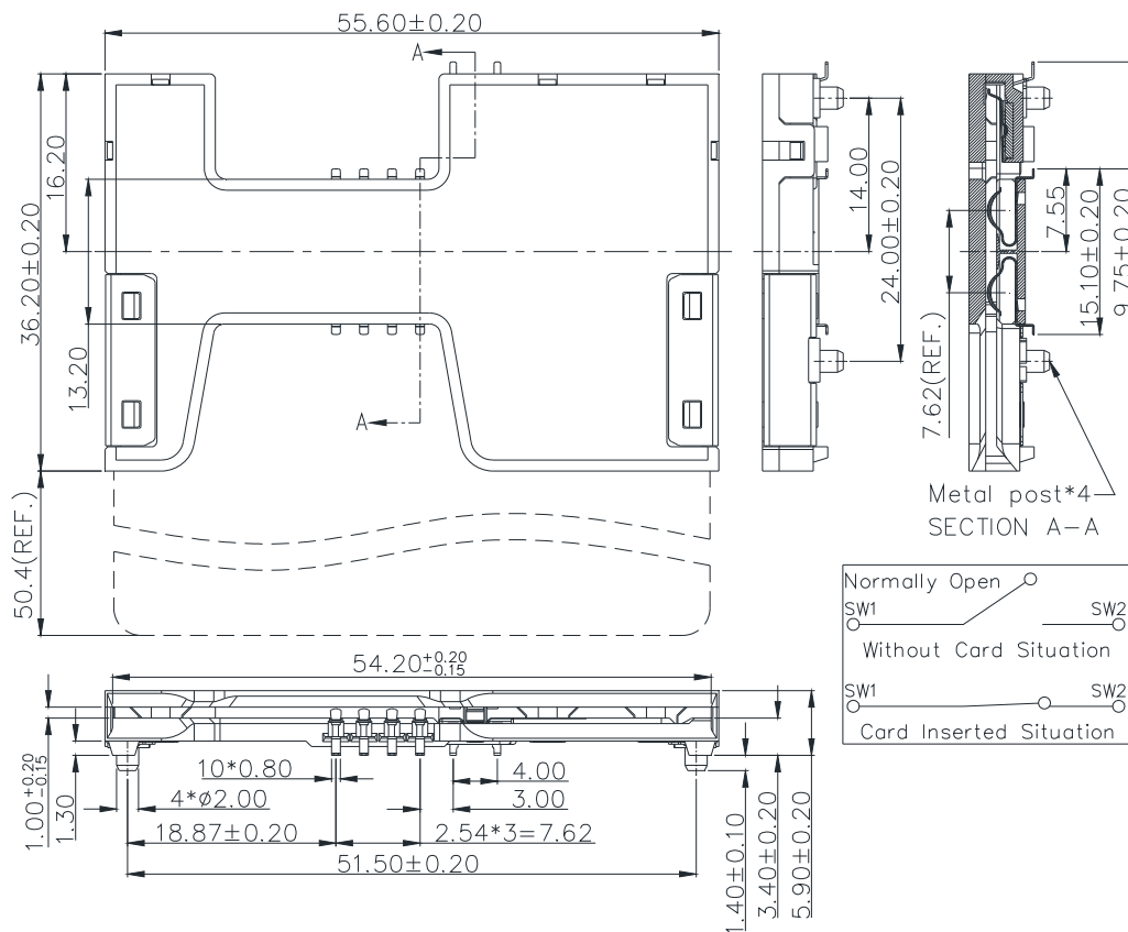
Unit: mm; Tolerances: \pm 0.15 mm Figure 5.1 Mechanical Outline dimension
