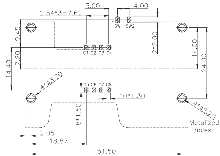
Unit: mm; Tolerances: \pm 0.05 mm Figure 5.2 Reference dimension for PCB layout
