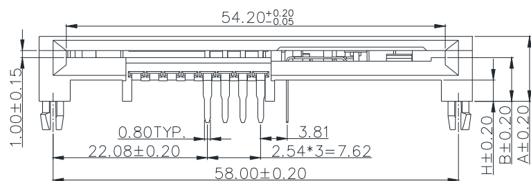
Unit: mm; Tolerances: \pm 0.15 mm Figure 5.1 Mechanical Outline dimension
