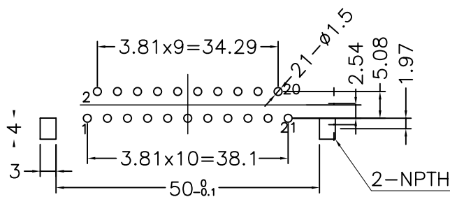
PCB HOLE PATTEN
