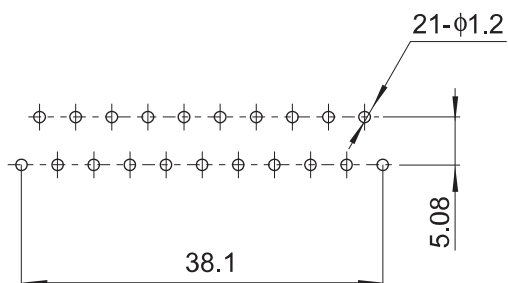
PCB HOLE PATTERN
