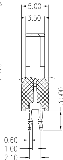
DETAIL A SCALE 2:1
